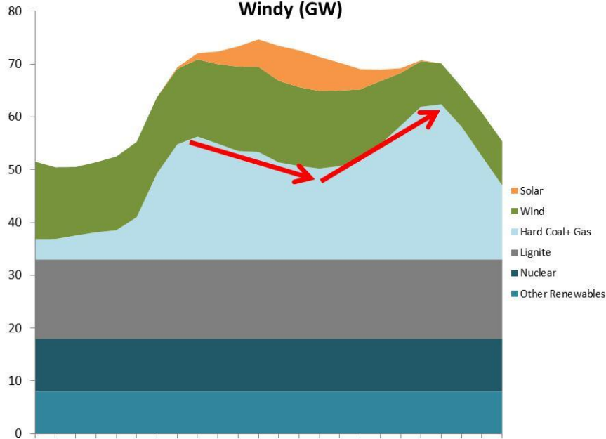
German Power Production Stack September 2011 - Windy (GW)
