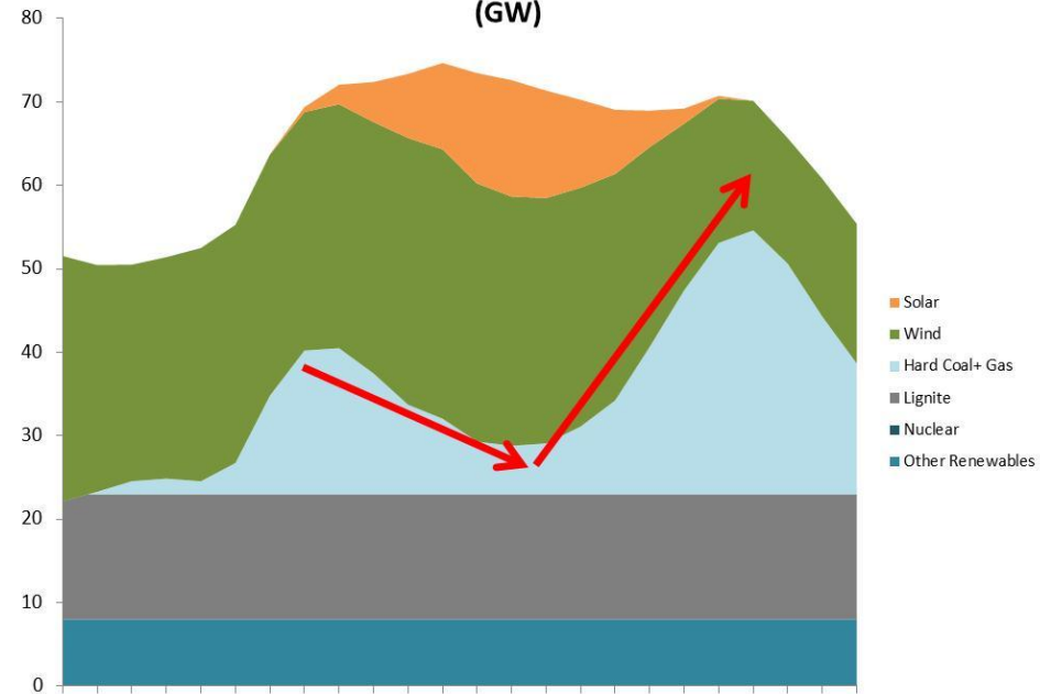
German Power Production Stack September 2025 - Windy (GW)
